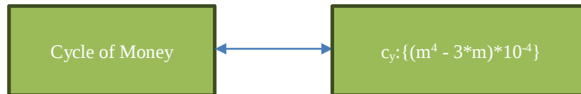
Figure 1: Cycle of money for c_y: \{(m^4 - 3*m)*10^{-4}\}
